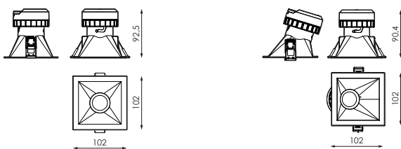
LIGHT ENGINE + ACCESSORY SQ 60° SYMMETRICAL
