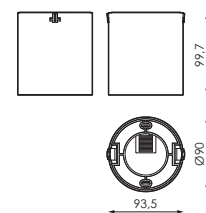
LIGHT ENGINE + ACCESSORY SURFACE
