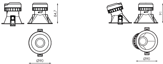
LIGHT ENGINE + ACCESSORY CL SYMMETRICAL 60°
